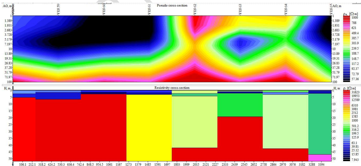
Figure 14: Pseudo cross-section and Resistivity cross-section of Profile 6 in the study area.
