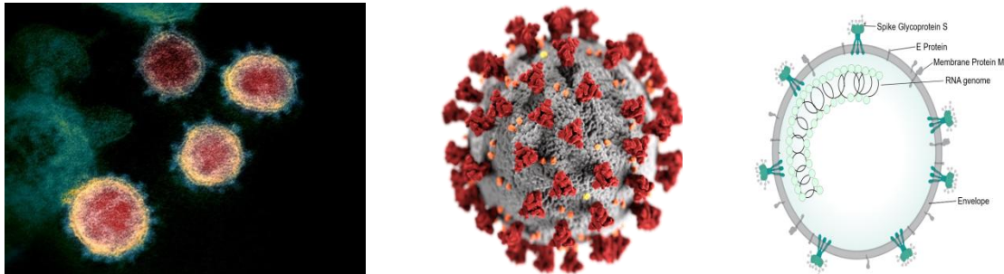
Figure 1: (a) Electron micrograph of SARS-CoV-2 virions with visible coronae (b). Illustration of a SARS-CoV-2 virion (c). Structure of a SARS-CoV virion.
