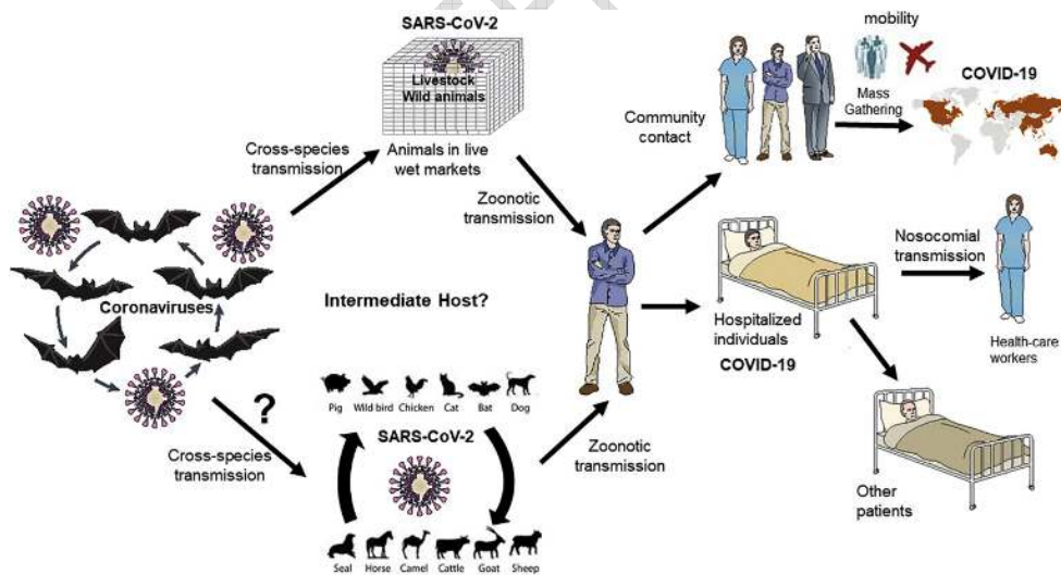
Fig. 2. The emergence of SARS-CoV-2 and the outbreak of COVID-19. The figure depicts a hypothesized origin of the virus and a generalised route of transmission of the epidemic zoonotic coronavirus. [11].
